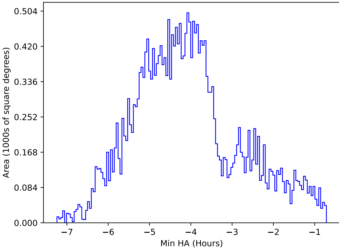
ddf_loaded_fl4_v3.4_10yrs All sky z band: Min HA
