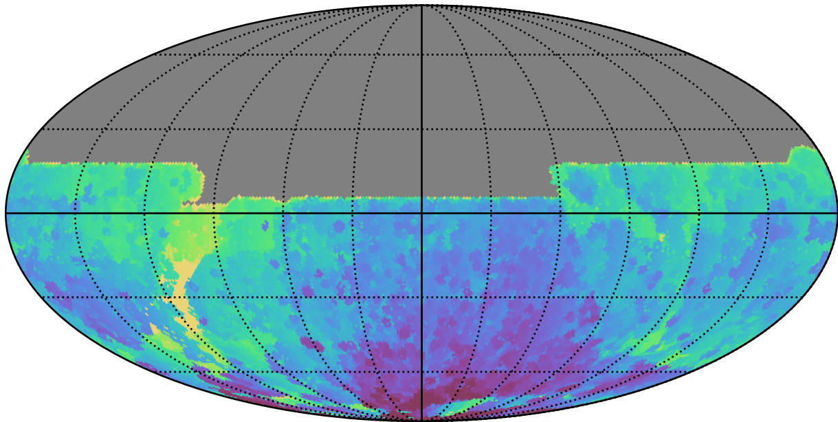
ddf_loaded_fl4_v3.4_10yrs All sky y band: Min HA
