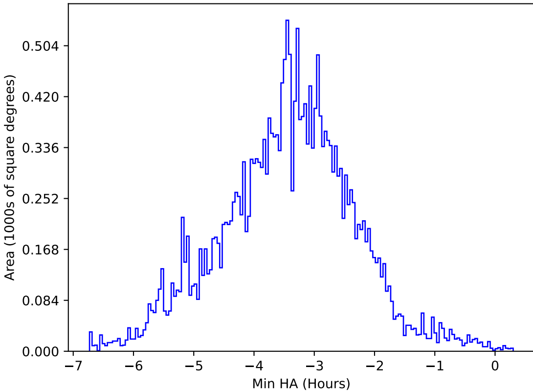
ddf_loaded_fl4_v3.4_10yrs All sky y band: Min HA
