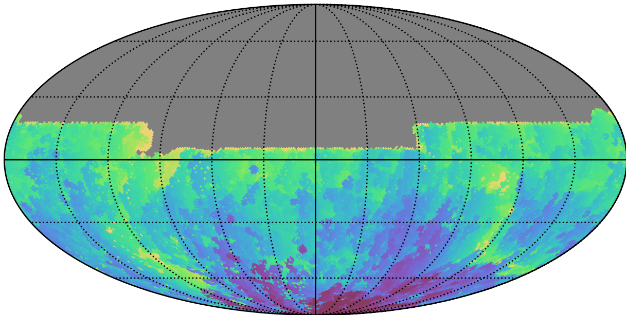
ddf_loaded_fl4_v3.4_10yrs All sky u band: Min HA
