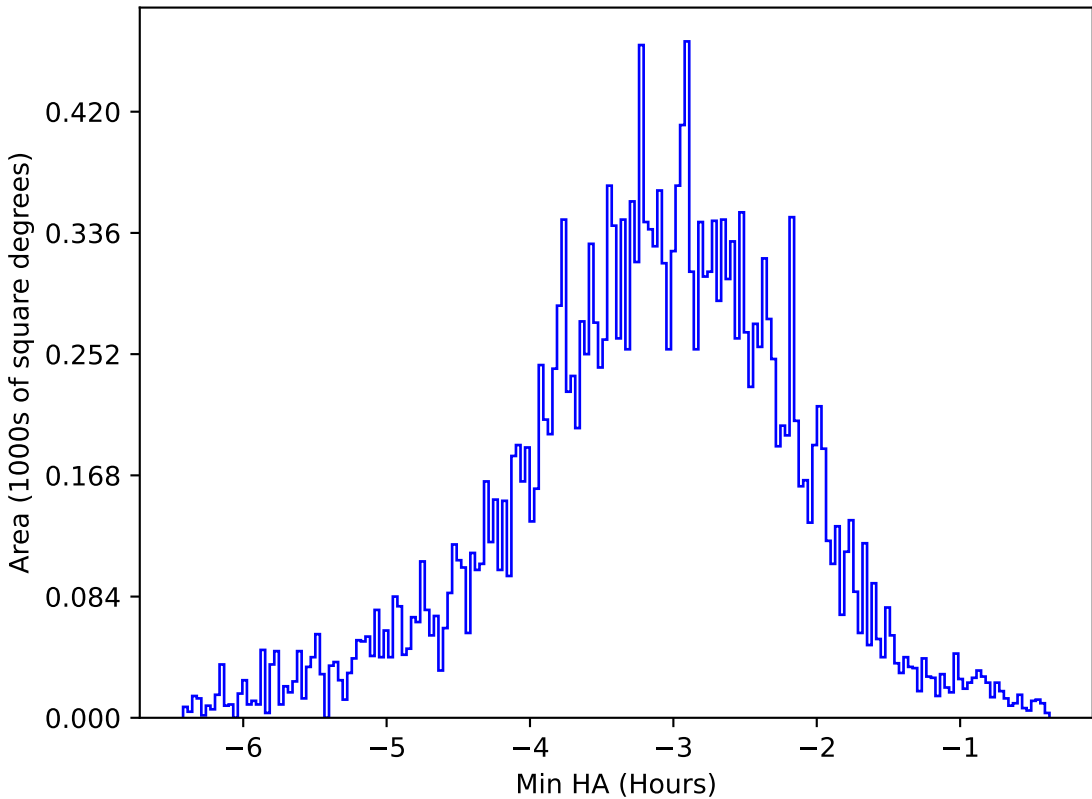
ddf_loaded_fl4_v3.4_10yrs All sky u band: Min HA
