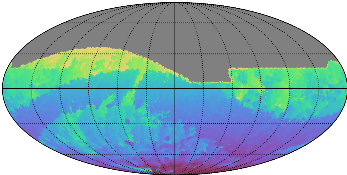
ddf_loaded_fl4_v3.4_10yrs All sky r band: Min HA
