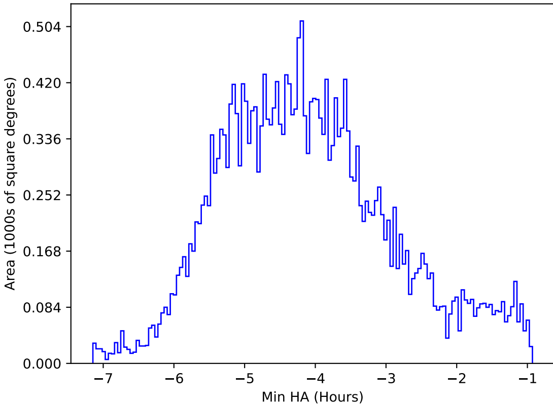
ddf_loaded_fl4_v3.4_10yrs All sky r band: Min HA
