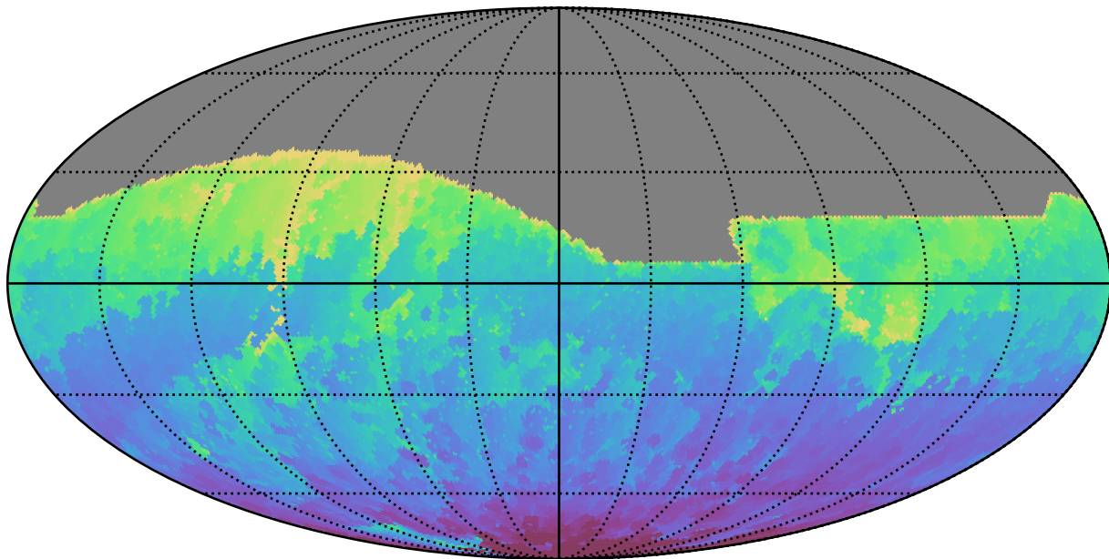
ddf_loaded_fl4_v3.4_10yrs All sky i band: Min HA
