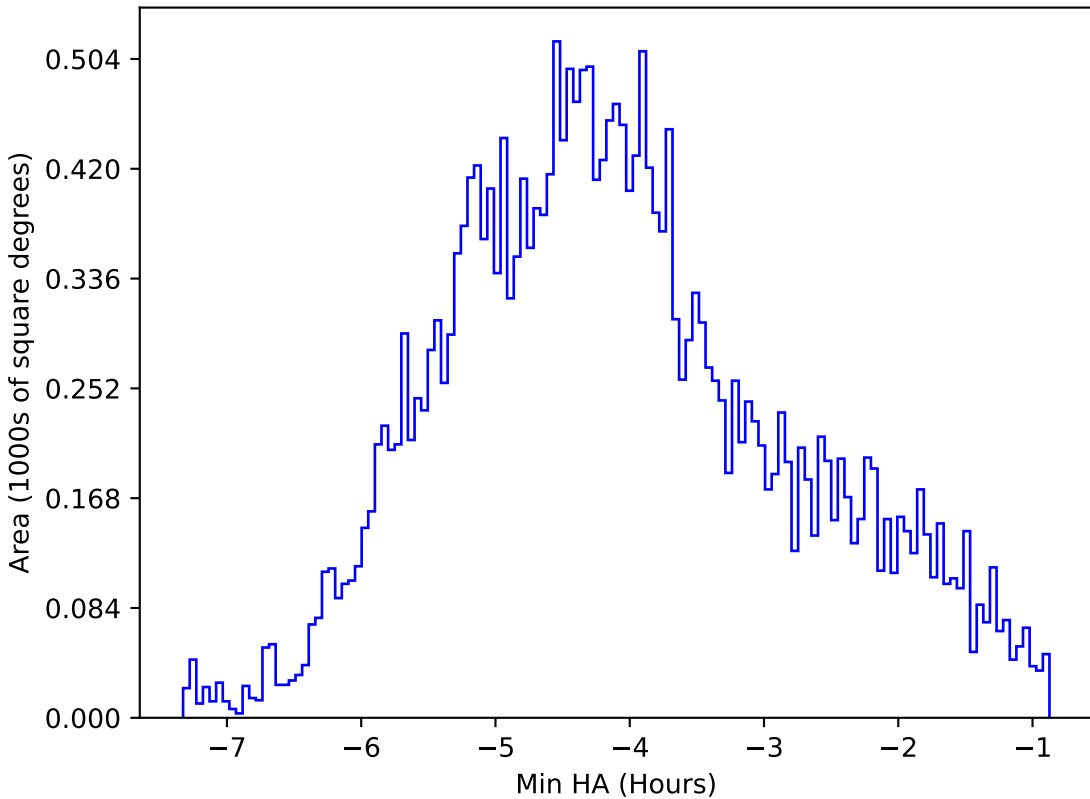
ddf_loaded_fl4_v3.4_10yrs All sky i band: Min HA
