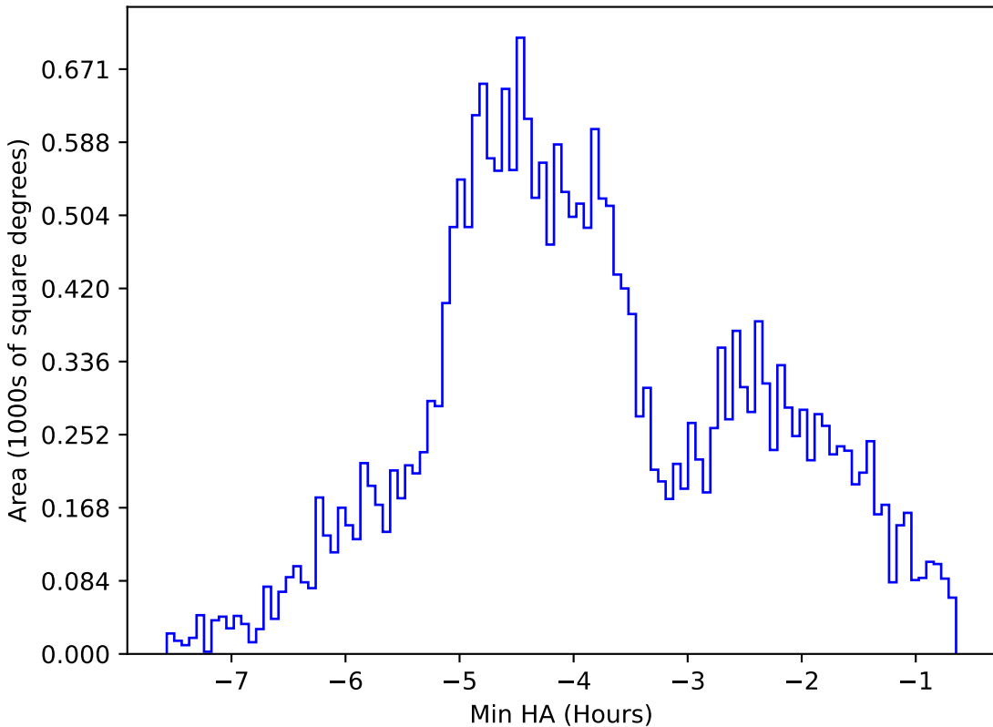
ddf_loaded_fl4_v3.4_10yrs All sky g band: Min HA
