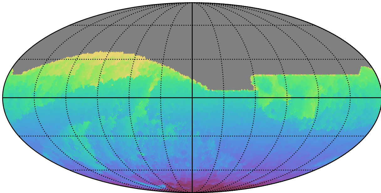
ddf_loaded_fl4_v3.4_10yrs All sky all bands: Min HA
