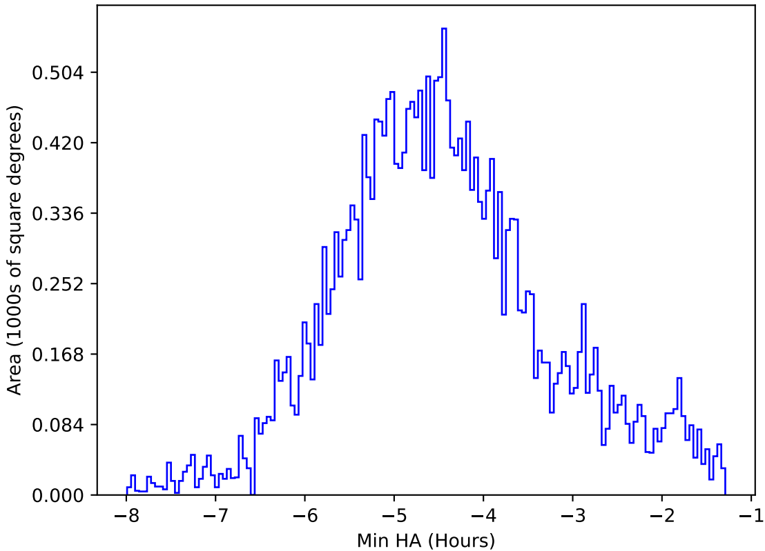
ddf_loaded_fl4_v3.4_10yrs All sky all bands: Min HA
