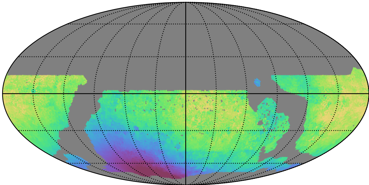
ddf_loaded_fl4_v3.4_10yrs WFD y band: Median solarElong
