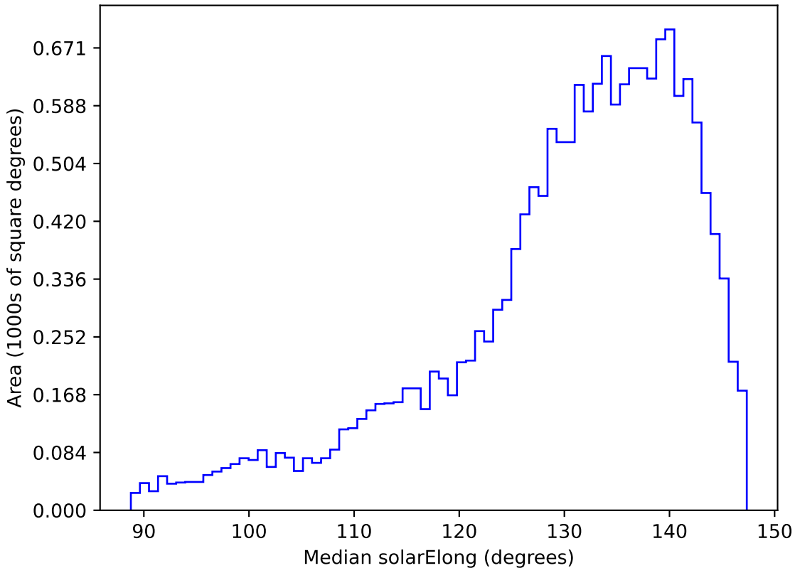
ddf_loaded_fl4_v3.4_10yrs WFD y band: Median solarElong
