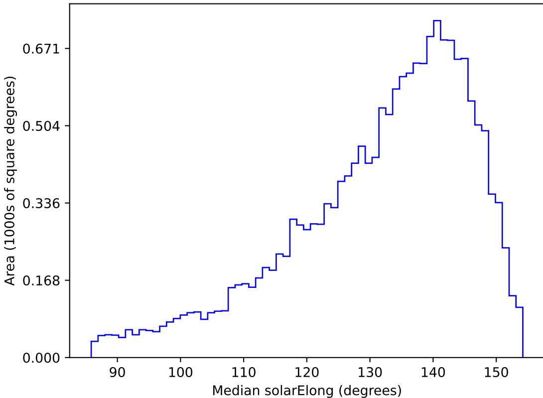
ddf_loaded_fl4_v3.4_10yrs WFD u band: Median solarElong
