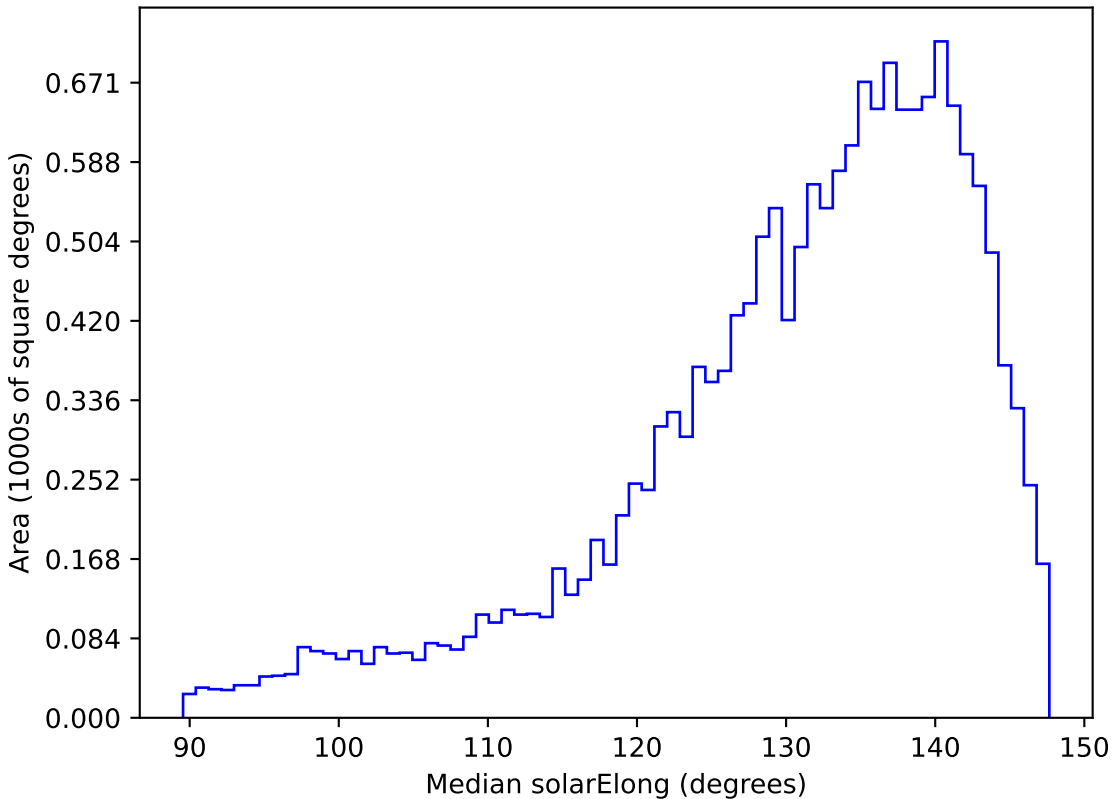
ddf_loaded_fl4_v3.4_10yrs WFD r band: Median solarElong
