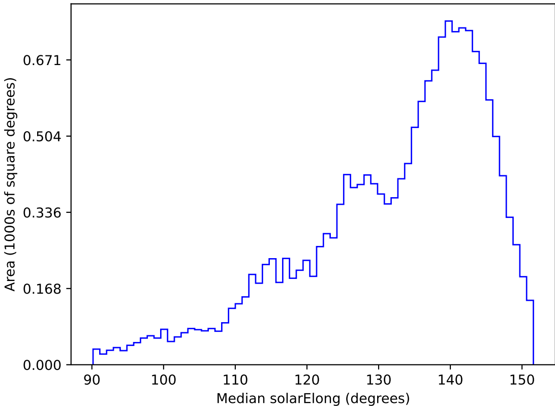
ddf_loaded_fl4_v3.4_10yrs WFD g band: Median solarElong
