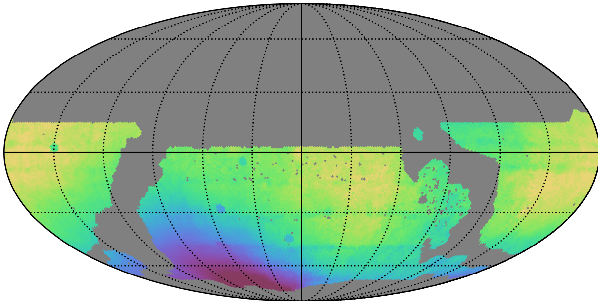
ddf_loaded_fl4_v3.4_10yrs WFD all bands: Median solarElong
