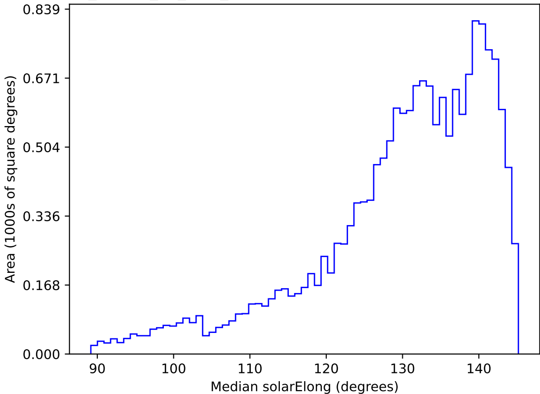
ddf_loaded_fl4_v3.4_10yrs WFD all bands: Median solarElong
