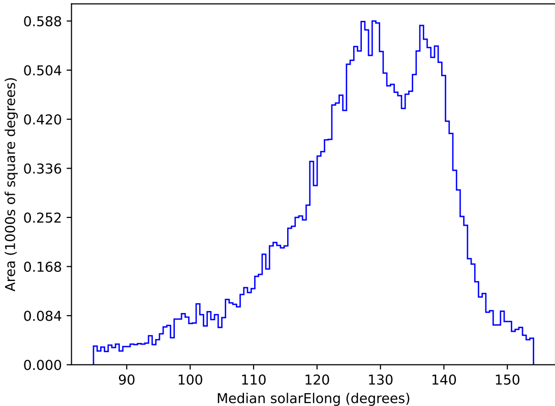
ddf_loaded_fl4_v3.4_10yrs All sky z band: Median solarElong
