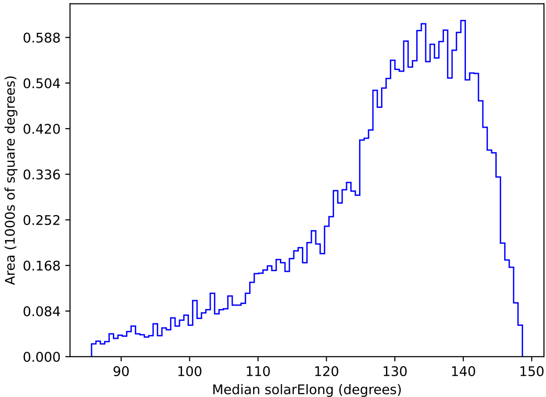
ddf_loaded_fl4_v3.4_10yrs All sky y band: Median solarElong
