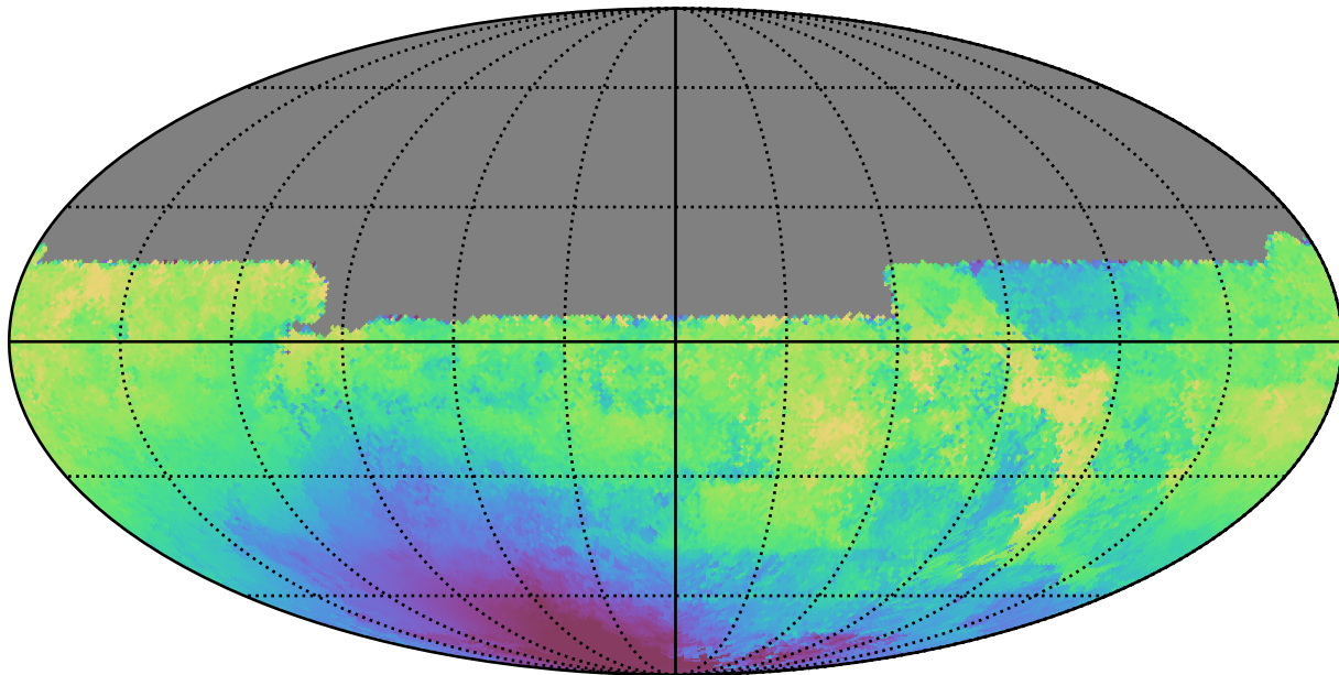
ddf_loaded_fl4_v3.4_10yrs All sky u band: Median solarElong
