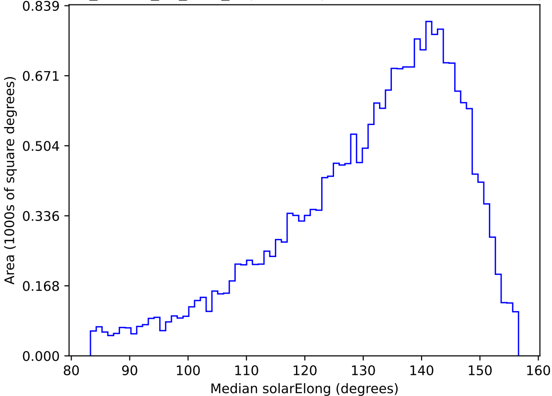
ddf_loaded_fl4_v3.4_10yrs All sky u band: Median solarElong
