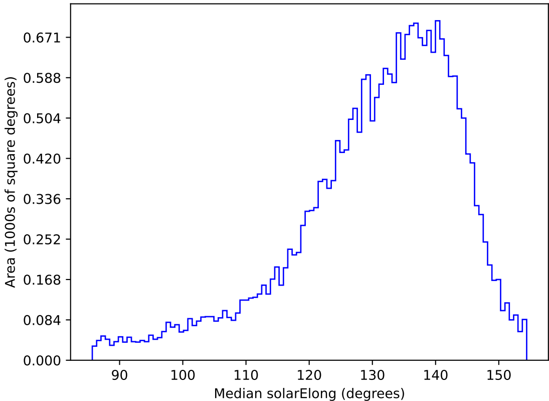
ddf_loaded_fl4_v3.4_10yrs All sky r band: Median solarElong
