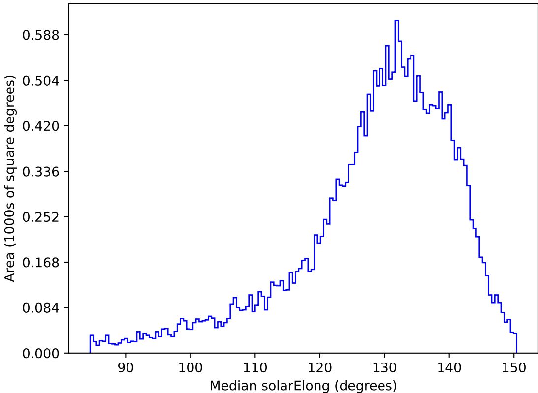
ddf_loaded_fl4_v3.4_10yrs All sky i band: Median solarElong
