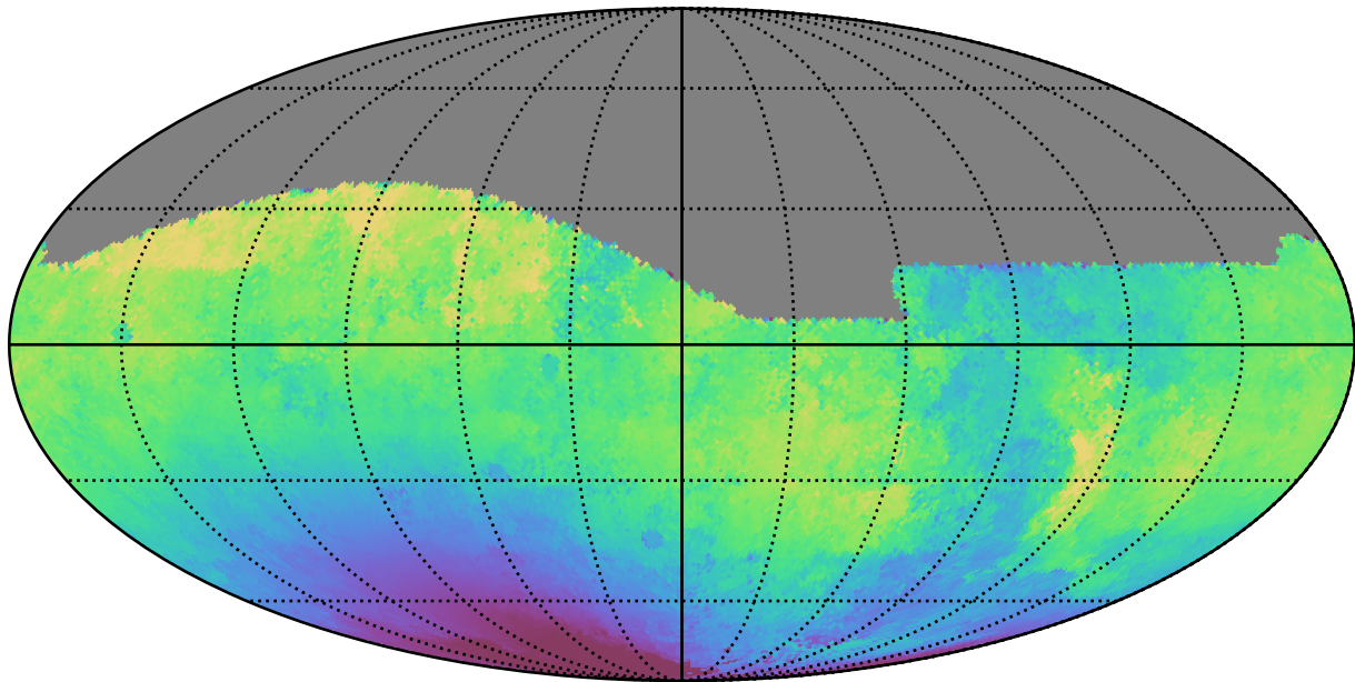
ddf_loaded_fl4_v3.4_10yrs All sky g band: Median solarElong
