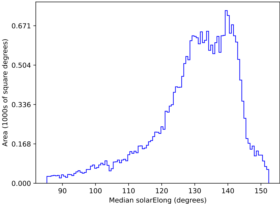
ddf_loaded_fl4_v3.4_10yrs All sky all bands: Median solarElong
