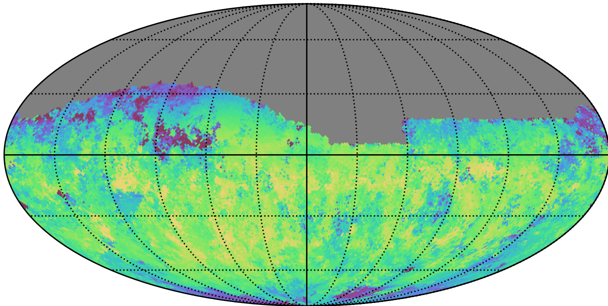
ddf_loaded_fl4_v3.4_10yrs Yr 1 z band: Median skyBrightness
