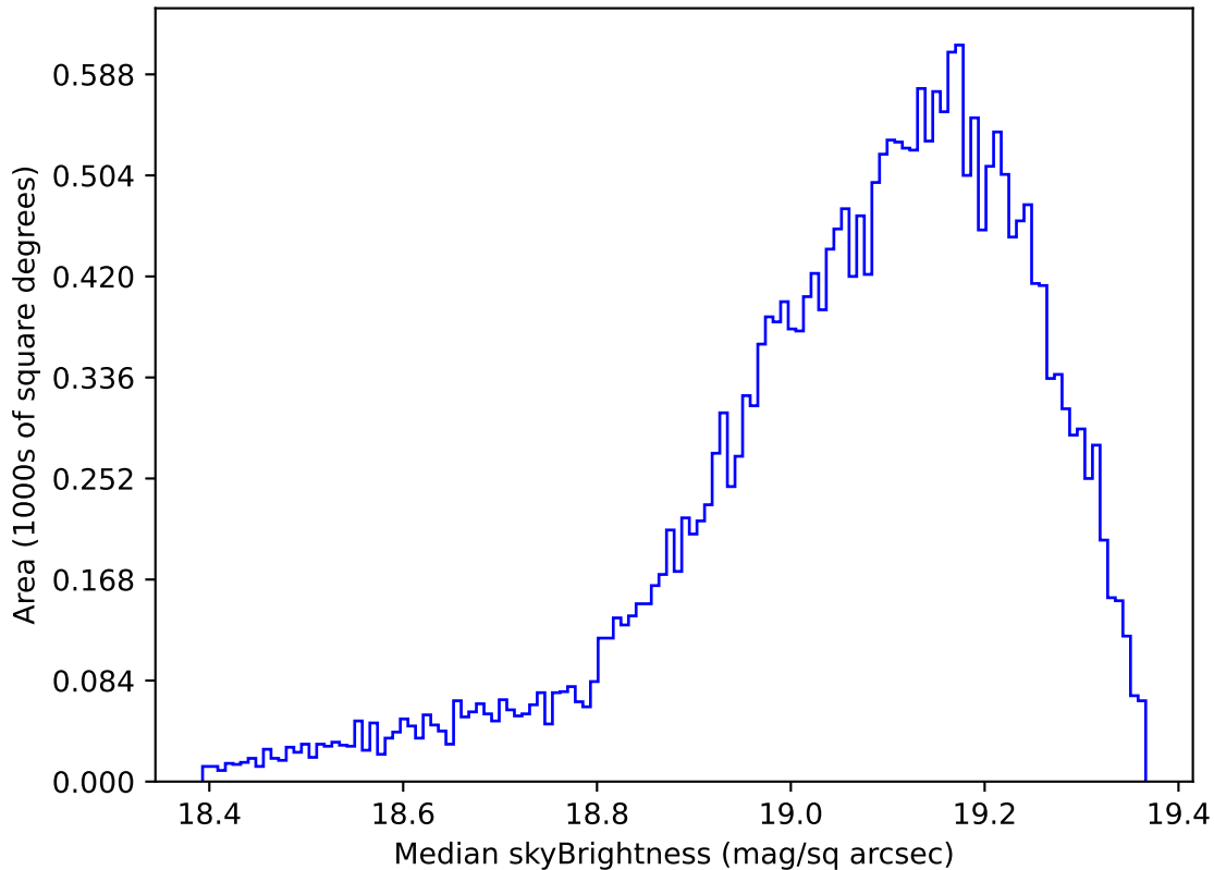
ddf_loaded_fl4_v3.4_10yrs Yr 1 z band: Median skyBrightness
