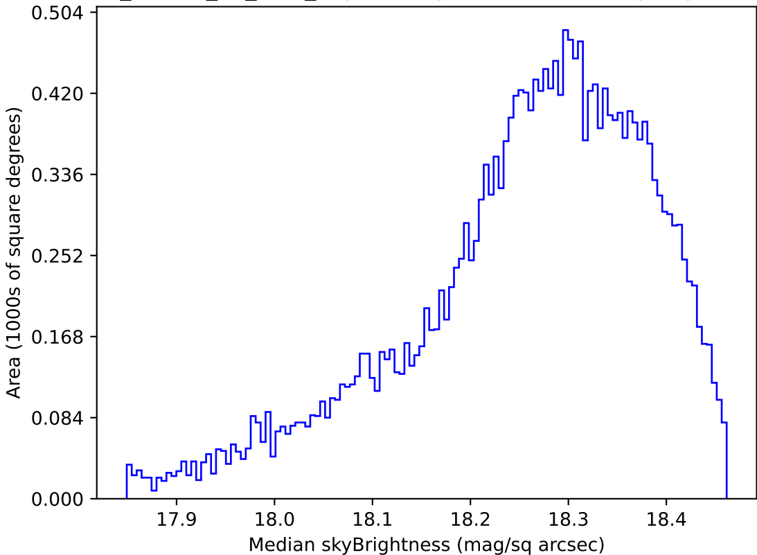
ddf_loaded_fl4_v3.4_10yrs Yr 1 y band: Median skyBrightness
