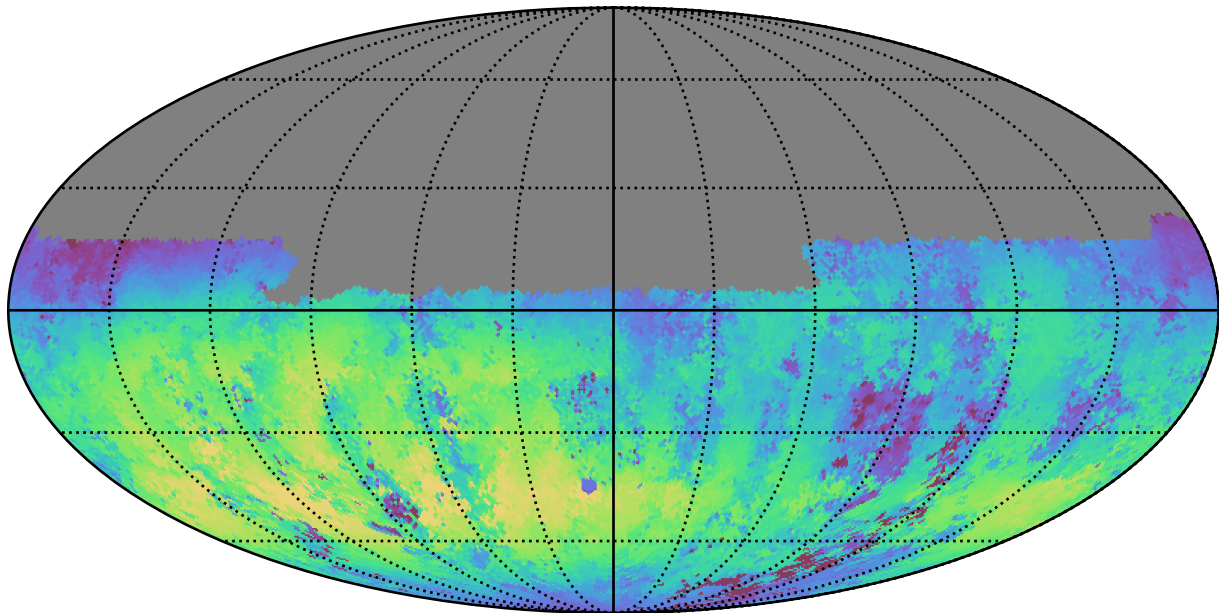
ddf_loaded_fl4_v3.4_10yrs Yr 1 u band: Median skyBrightness
