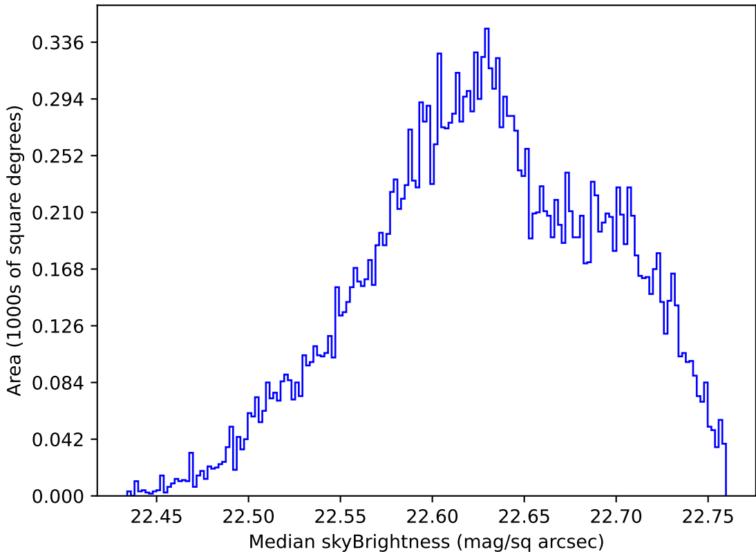
ddf_loaded_fl4_v3.4_10yrs Yr 1 u band: Median skyBrightness
