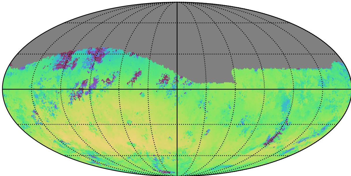
ddf_loaded_fl4_v3.4_10yrs Yr 1 r band: Median skyBrightness
