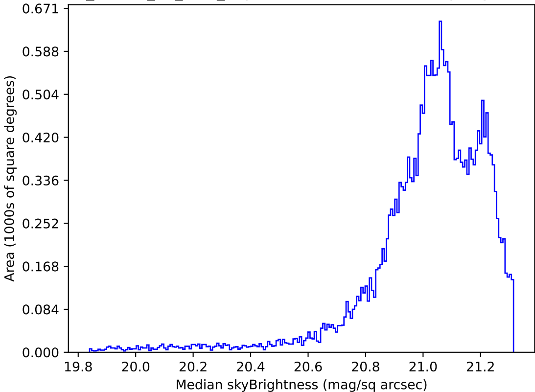
ddf_loaded_fl4_v3.4_10yrs Yr 1 r band: Median skyBrightness
