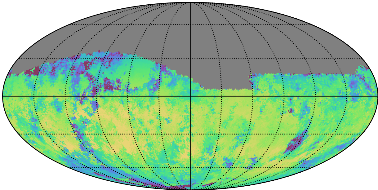
ddf_loaded_fl4_v3.4_10yrs Yr 1 i band: Median skyBrightness
