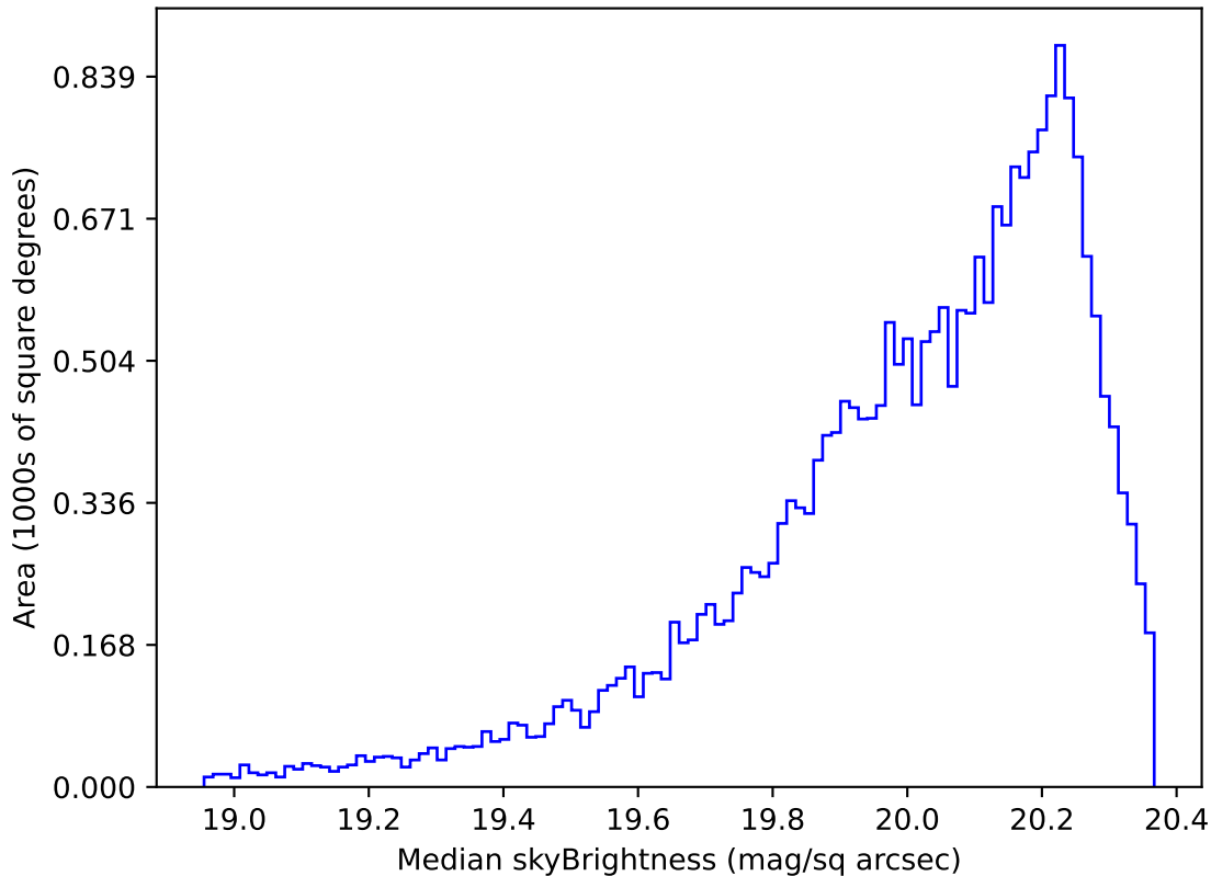
ddf_loaded_fl4_v3.4_10yrs Yr 1 i band: Median skyBrightness
