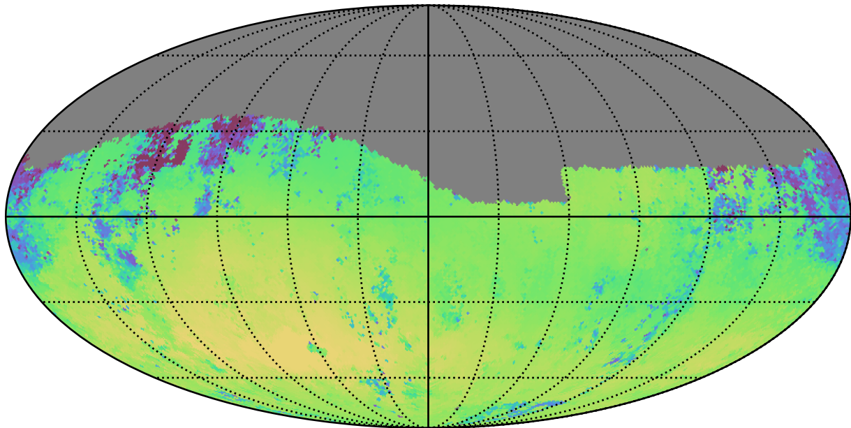
ddf_loaded_fl4_v3.4_10yrs Yr 1 g band: Median skyBrightness
