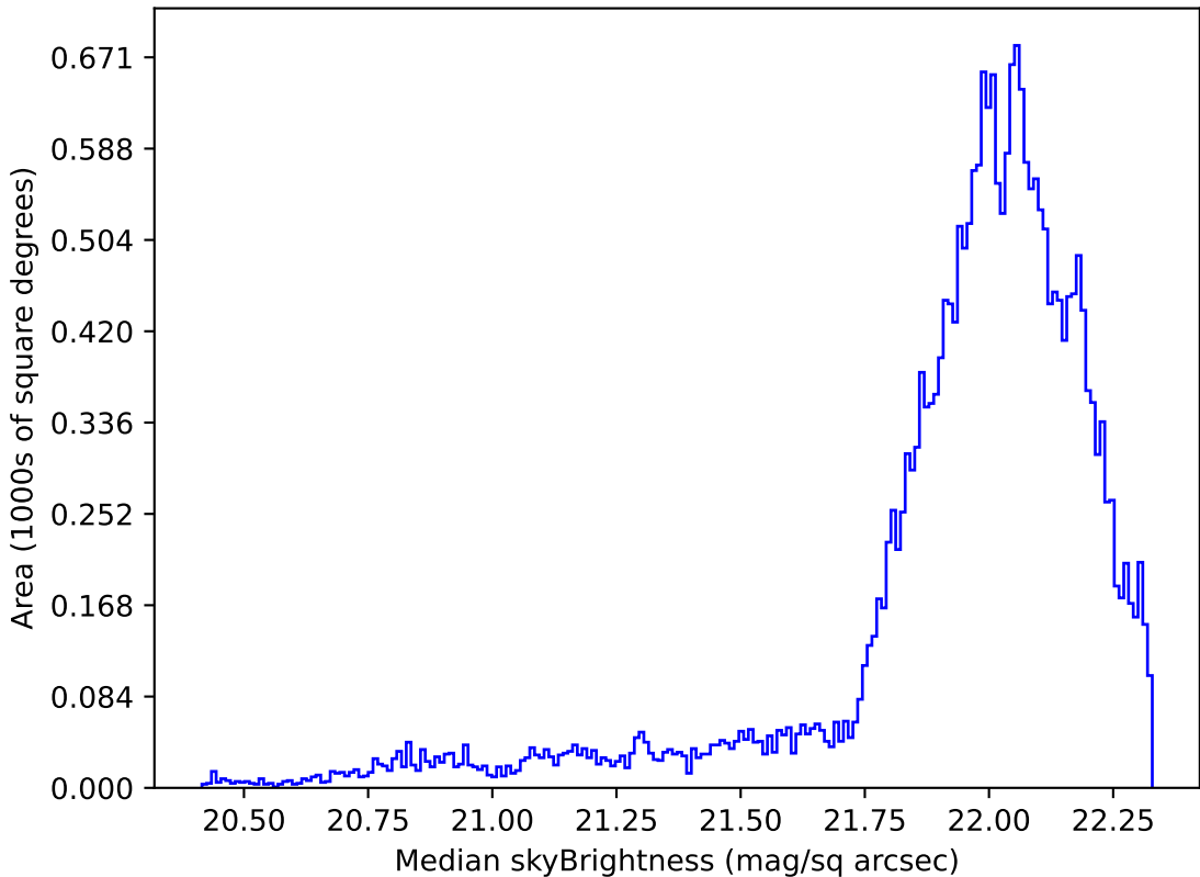
ddf_loaded_fl4_v3.4_10yrs Yr 1 g band: Median skyBrightness
