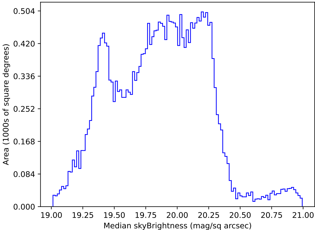
ddf_loaded_fl4_v3.4_10yrs Yr 1 all bands: Median skyBrightness
