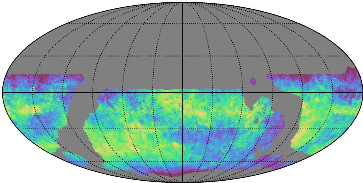
ddf_loaded_fl4_v3.4_10yrs WFD z band: Median skyBrightness
