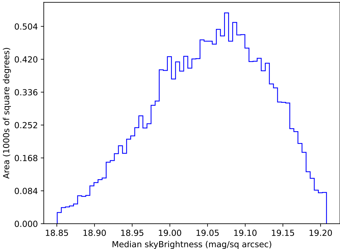
ddf_loaded_fl4_v3.4_10yrs WFD z band: Median skyBrightness
