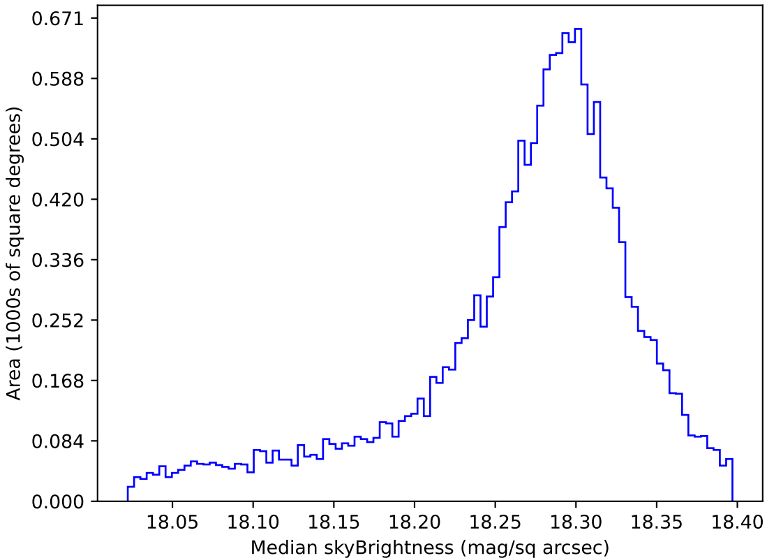
ddf_loaded_fl4_v3.4_10yrs WFD y band: Median skyBrightness
