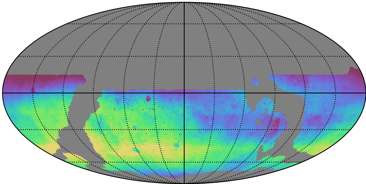
ddf_loaded_fl4_v3.4_10yrs WFD u band: Median skyBrightness
