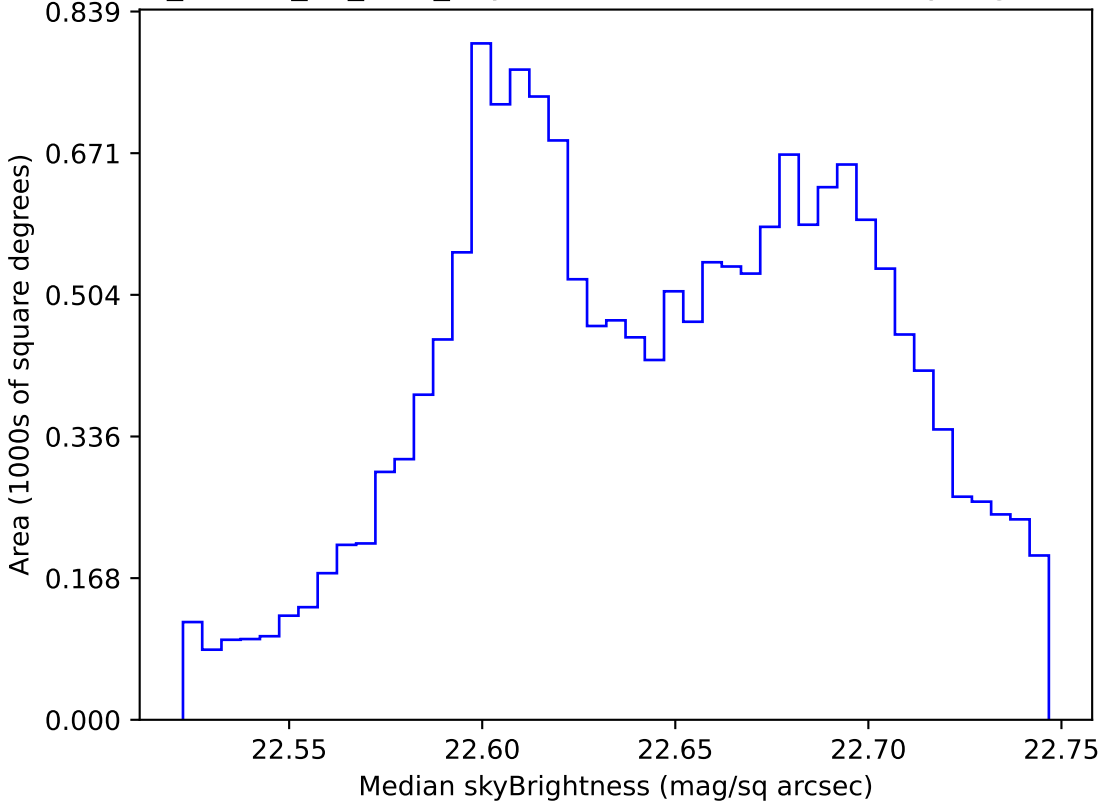
ddf_loaded_fl4_v3.4_10yrs WFD u band: Median skyBrightness
