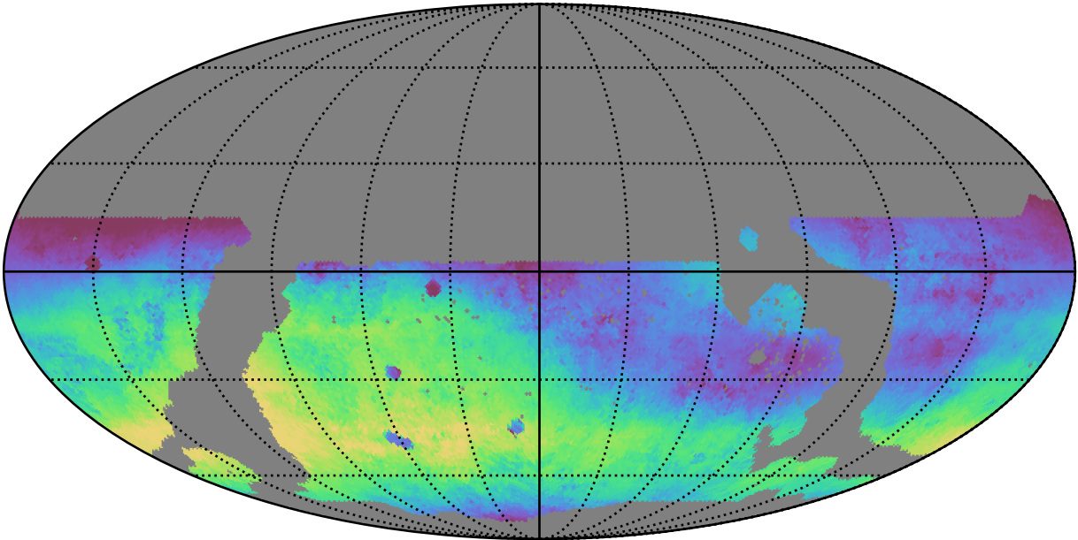
ddf_loaded_fl4_v3.4_10yrs WFD r band: Median skyBrightness
