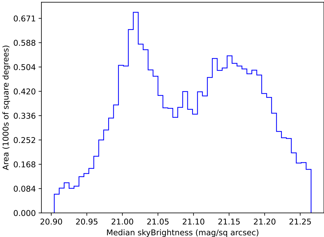
ddf_loaded_fl4_v3.4_10yrs WFD r band: Median skyBrightness
