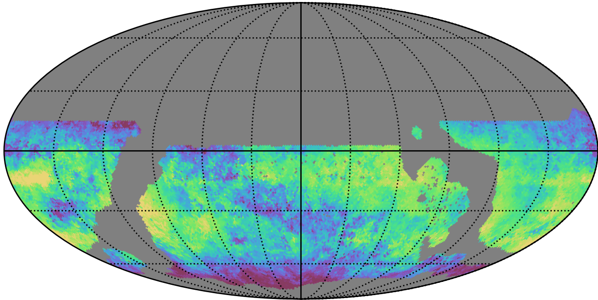
ddf_loaded_fl4_v3.4_10yrs WFD i band: Median skyBrightness
