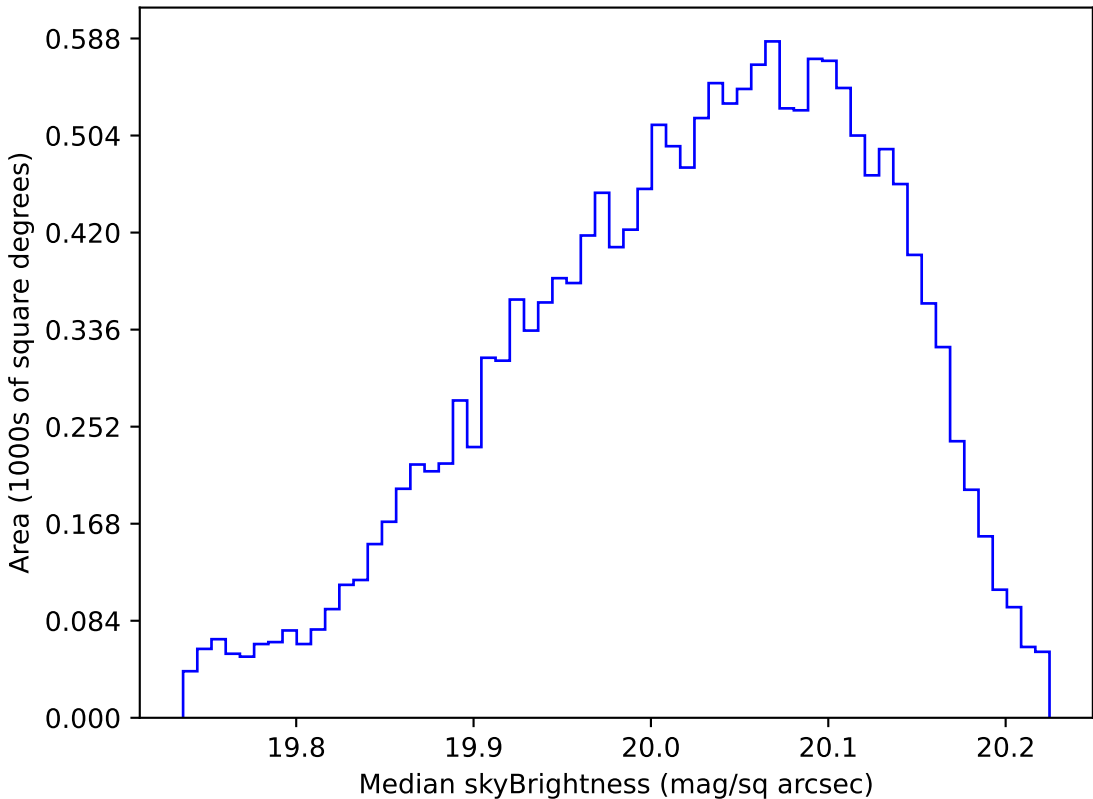
ddf_loaded_fl4_v3.4_10yrs WFD i band: Median skyBrightness
