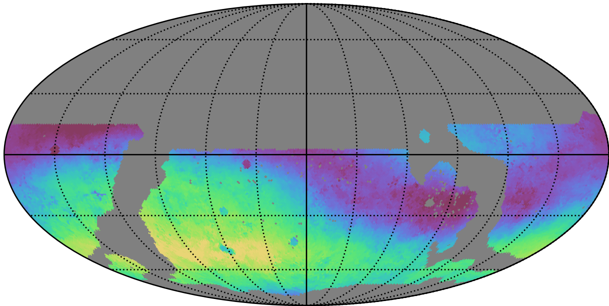
ddf_loaded_fl4_v3.4_10yrs WFD g band: Median skyBrightness
