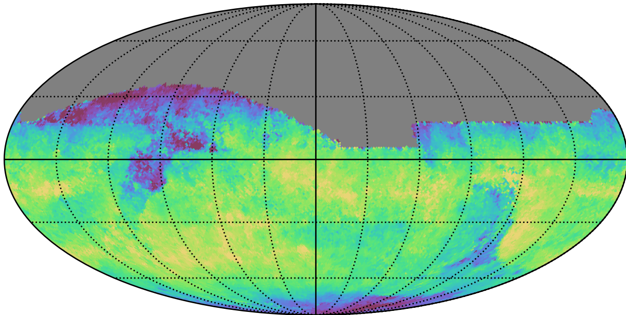
ddf_loaded_fl4_v3.4_10yrs All sky z band: Median skyBrightness
